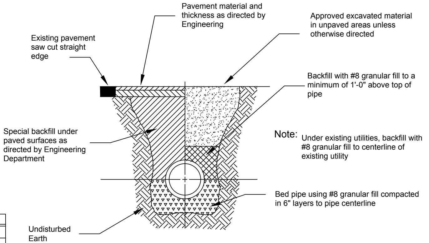
TRENCH DETAIL FOR SEWER MAINS
